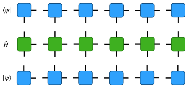
Fig. 2: The expectation value of an operator \hat{H} is shown in tensor diagram notation for a 6-site system. When contracted, this would give \langle \hat{H} \rangle , or the energy E if \hat{H} is the Hamiltonian. The wavefunction on the bottom row alone would be represented as in the text (Eq. 1), which is far more intricate.
