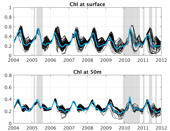
Fig. 9: Ensemble of model predictions (black curves) by a simple multi-layer perceptron (from Flux.jl) trained to predict Chlorophyll concentration (present in green algae and marine microbes) from environmental variables (T, S, but also oxygen, optical backscatter, and solar radiation). The blue line is the model ground truth that we seek to estimate, and was obtained through proper spatial averaging of the gridded data set from which the training data itself was generated.
