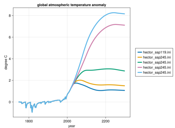
Fig. 10: Prediction of global warming based on different scenarios, called Shared Socioeconomic Pathways (SSPs), as defined by the Intergovernmental Panel on Climate Change (IPCC). These predictions were generated using the Hector model [13] via CLIMATEMODELS.JL.
