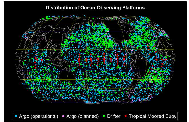
Fig. 1: Ocean robots that were collecting data on 2024/11/29 for three types of observations (blue, green, and red dots). Planned deployments of Argo profilers are also shown (purple dots). Data is from https://www.ocean-ops.org and queried via OCEANROBOTS.JL.
