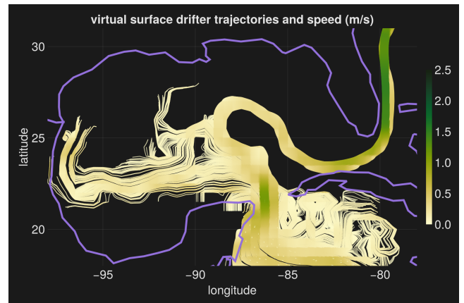
Fig. 7: Virtual drifter trajectories predicted using (1) just the climatological mean flow field estimated from drifters (Fig. 3, plus the corresponding northward component) and (2) DRIFTERS.JL to calculate trajectories.
