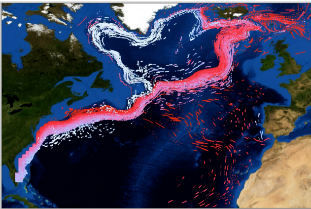
Fig. 11: Tracking Gulf Stream waters from Florida Strait to the subpolar gyre using virtual drifters that follow the three dimensional ocean circulation. Each dot color indicates the virtual drifter depth – red dots near the sea surface, while white dots are below 1500m depth.
