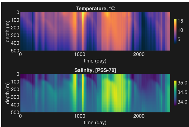
Fig. 5: Virtual Argo profiles predicted using the OCCA climatology, interpolated to the positions of the float shown in Fig. 4.
