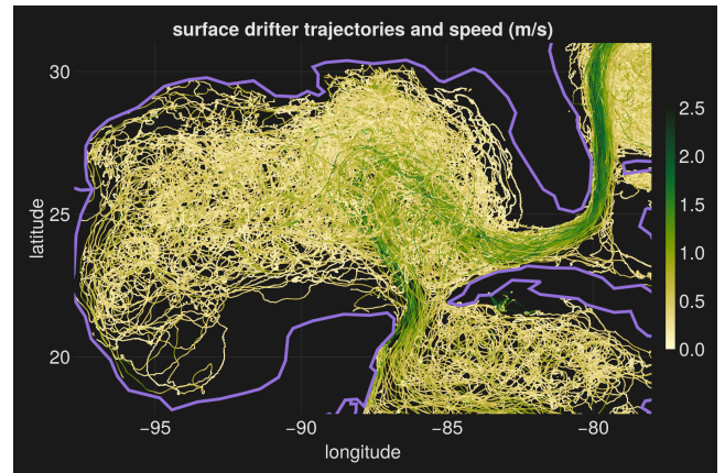
Fig. 6: Drifter trajectories in the Gulf of Mexico region. Large velocities highlight the path of the Gulf Stream, being fed by the loop current.
