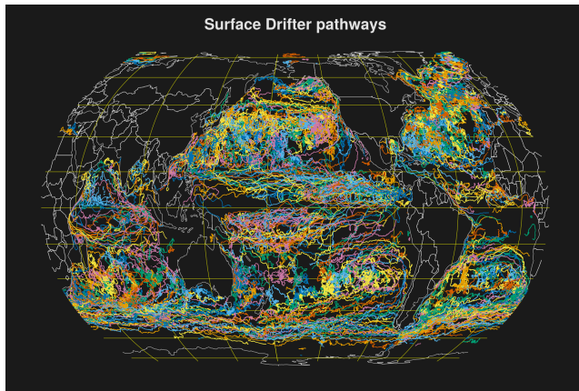
Fig. 2: A few of the ocean drifters (5% of 19396) that have been deployed to follow near surface ocean currents in the past.
