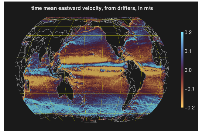
Fig. 3: Sample mean eastward velocity estimated from drifter data, with a grid resolution of 1/2 degree.
