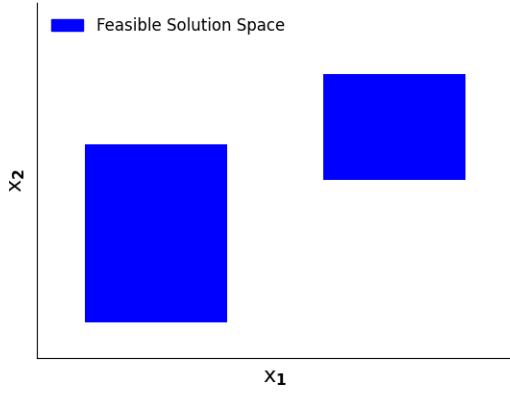
Fig. 1. Feasible solution space for example disjunction
