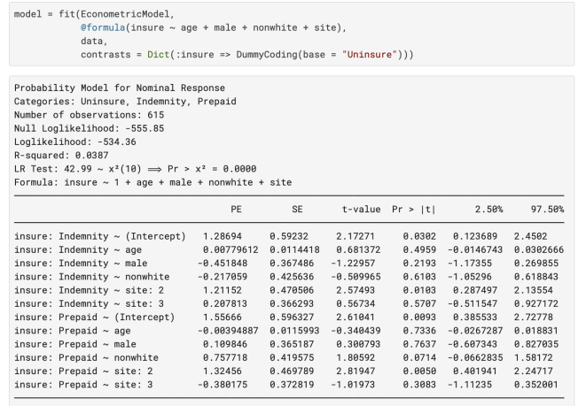
Fig. 5: Estimation of the multinomial logistic regression
