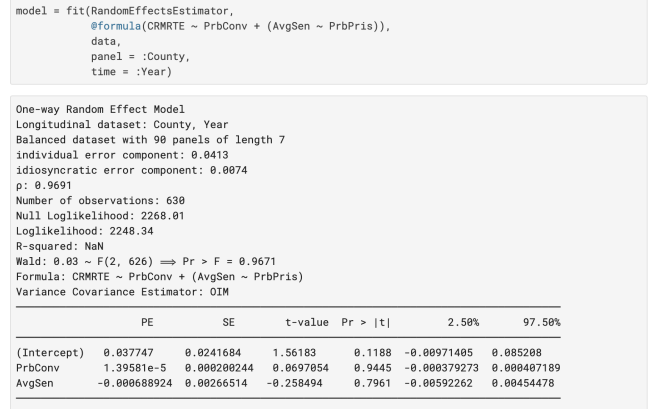
Fig. 4: Estimation of the random effects model
