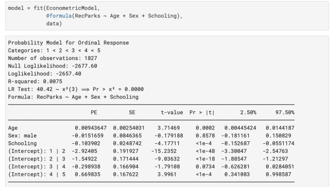
Fig. 6: Estimation of the proportional odds logistic regression
